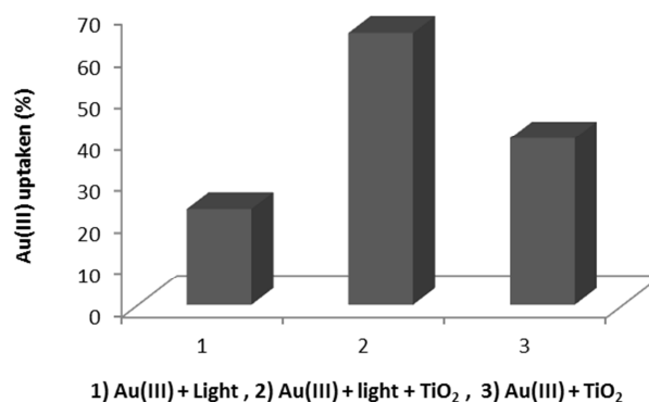
Fig. 2. The uptake of Au(III) from the solution by different processes.
