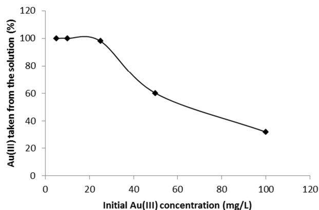
Fig. 5. The influence of Au(III) initial concentration.
